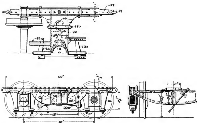
Figs. 4331-4333. Equalized Pedestal Tender Truck. American Locomotive Co.
